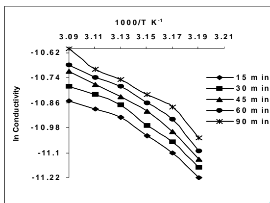
Figure (4) \ln s against (1000/T) for nano PbS films at Different Deposition time.
