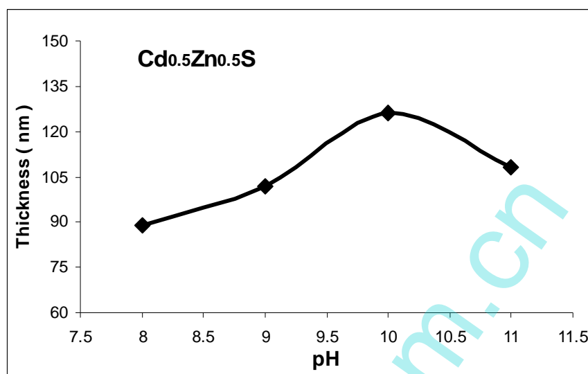
Figure (1) Influence of pH on Cd_{0.5}Zn_{0.5}S film thickness.
