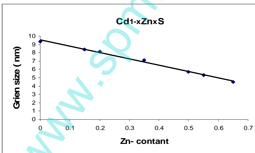
Figure (5) shows the variation of grain size versus Zn- content.
