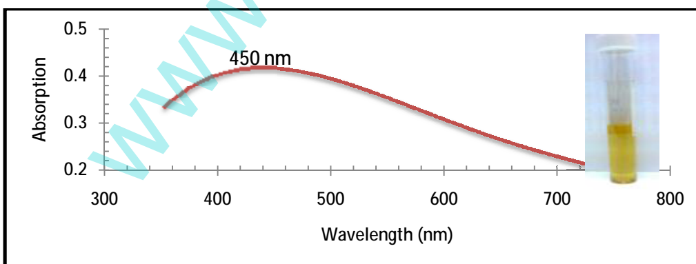
Figure (1) UV-VIS spectral and photo of Ag nanoparticles by chemical reduction AgNO 3 with TSC.
