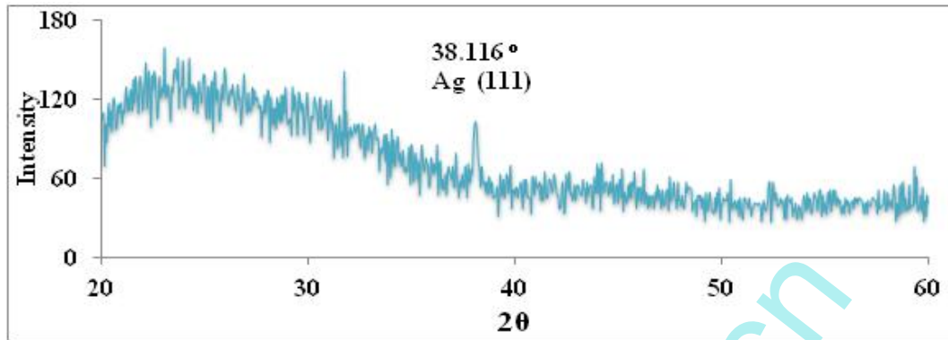
Figure (5) X-Ray diffraction of Ag nanoparticles was produced by chemical reduction \text{AgNO}_3 with \text{NaBH}_4 .
