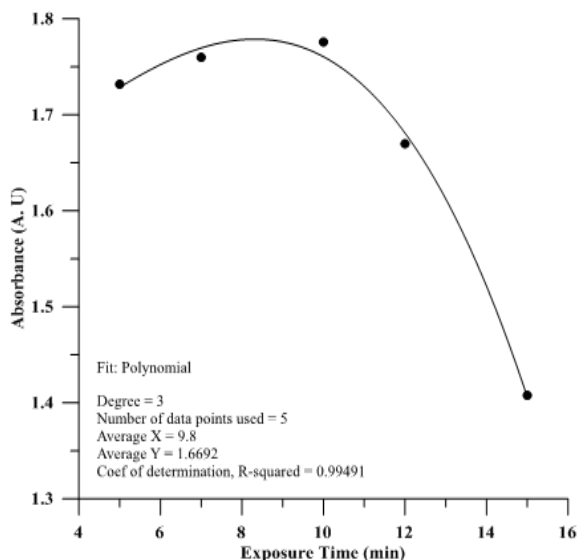
Figure 9 UV-Visible spectrums as function of exposure time
