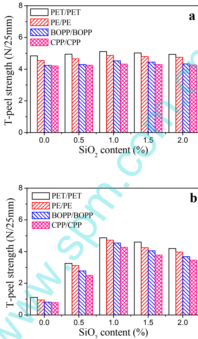
Fig.12 Effect of nano-SiO 2 content on adhesive property of SiO 2 /FWPU adhesive at (a) 25 0 C and (b) cooking at 120 0 C under high temperature atmosphere
