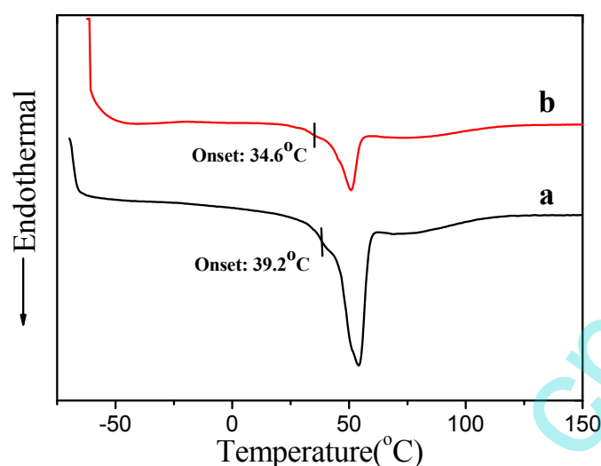
Fig. 3 DSC curves of waterborne polyurethane (a) pure WPU (b) SiO 2 /FWPU-15
