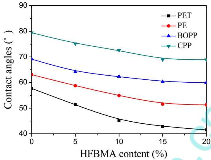
Fig. 5 The static contact angle of nanocomposite emulsions on the nonpolar polyolefin films
