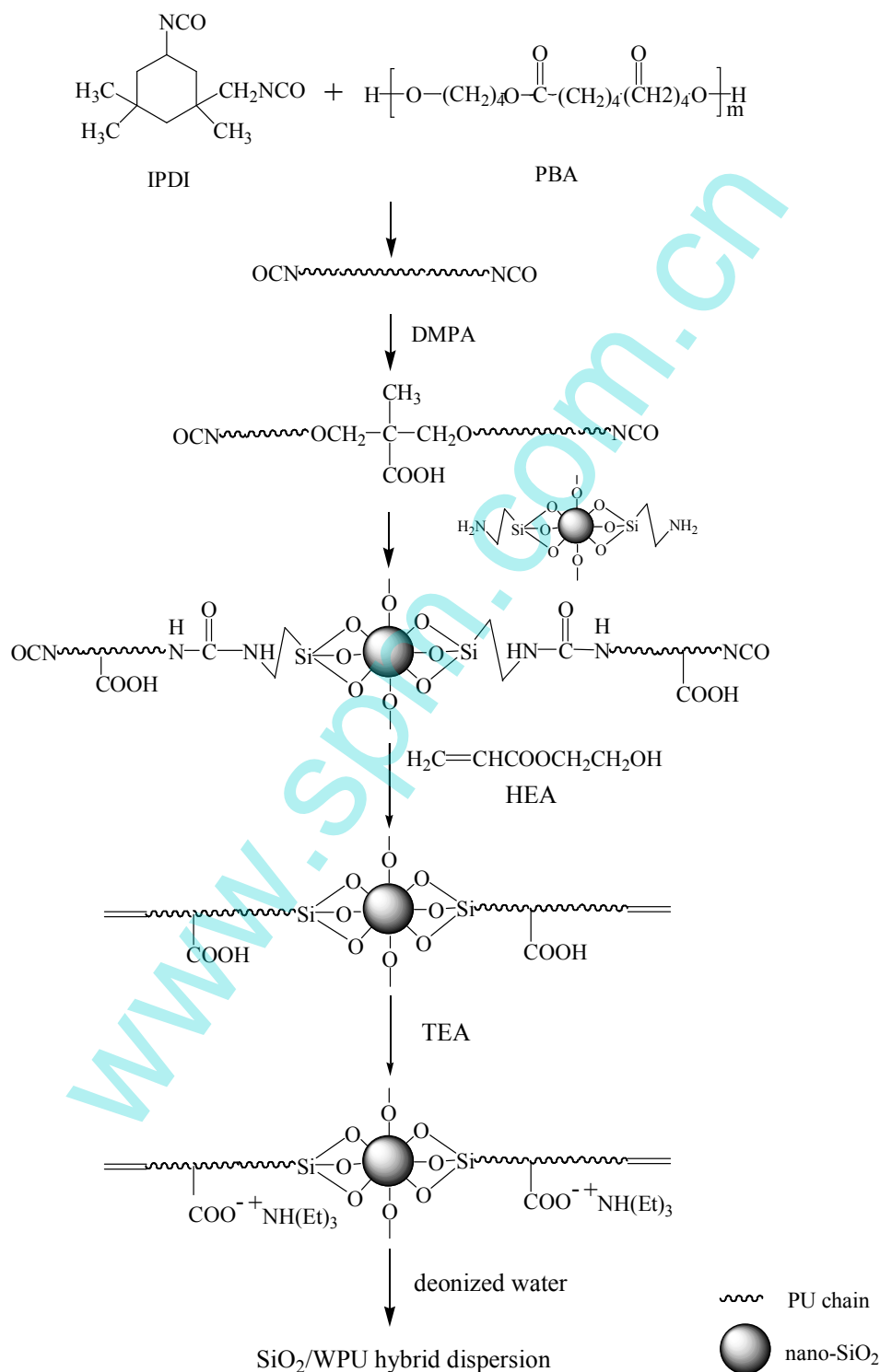
Fig.1 Flowchart of the preparation of SiO 2 /WPU hybrid dispersion
