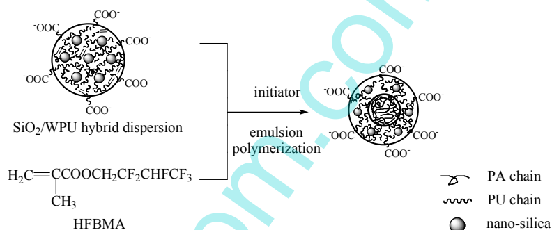
Fig.2 Schematic of the formation of SiO 2 /FWPU nanocomposite particle
