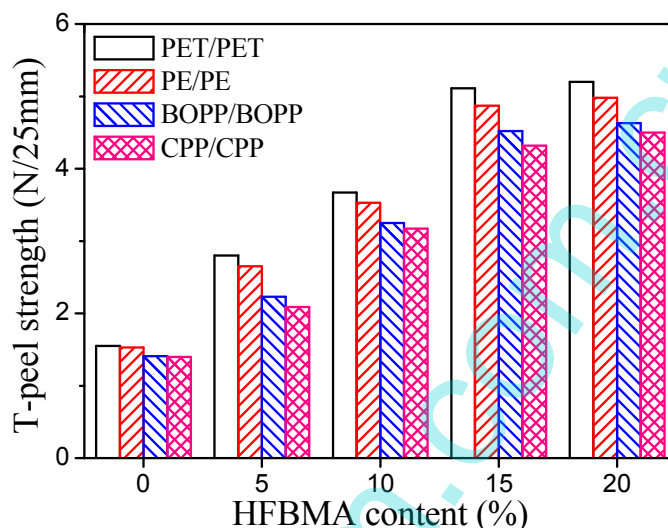
Fig.11 Effect of HFBMA content on adhesive property of SiO 2 /FWPU adhesive at 25 0 C
