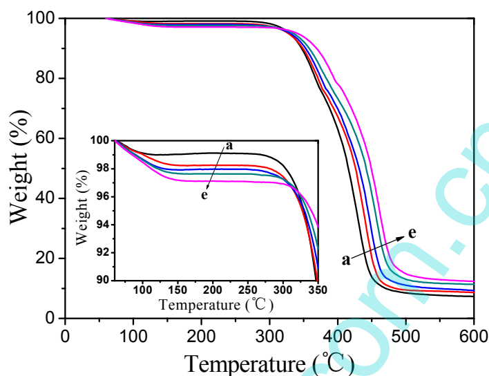
Fig. 9 TGA curves of the SiO 2 /FWPU composites with different SiO 2 content (a) 0% (b) 0.5% (c) 1% (d) 1.5% (e) 2%
