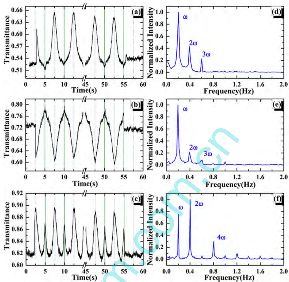
Figure 4. (a–c) are the modulated transmittance trajectories for selected mGO spots varied as the electric field E = E_0 \sin(\omega t) , respectively. The cycles with 5 s have been indicated by dash lines. (d–f) are the corresponding FFTs (normalized) for the transmittance of (a–c), respectively. The main harmonic signals have been labeled in frequency domain.
